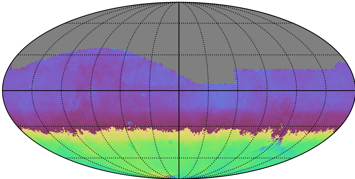
too_combined_s0.5_v3.4_10yrs All sky i band: AngleMean rotSkyPos
