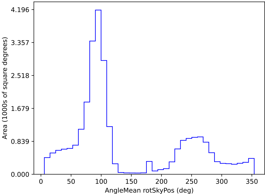
too_combined_s0.5_v3.4_10yrs All sky g band: AngleMean rotSkyPos
