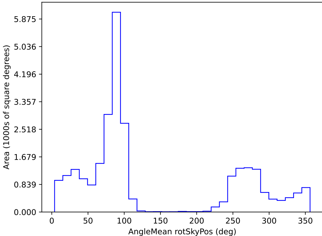
too_combined_s0.5_v3.4_10yrs All sky all bands: AngleMean rotSkyPos
