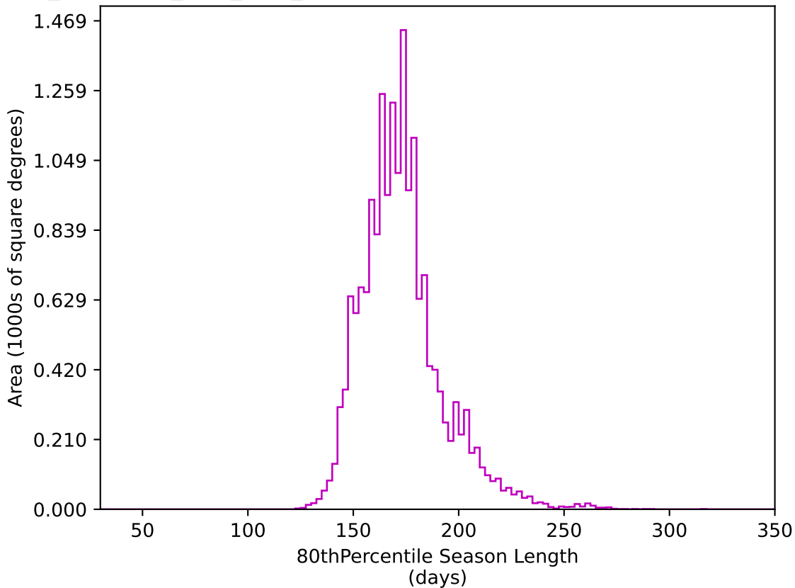
too_combined_s0.5_v3.4_10yrs WFD z band: 80thPercentile Season Length
