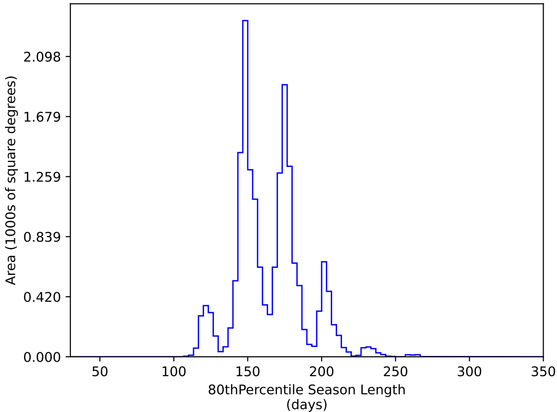
too_combined_s0.5_v3.4_10yrs WFD y band: 80thPercentile Season Length
