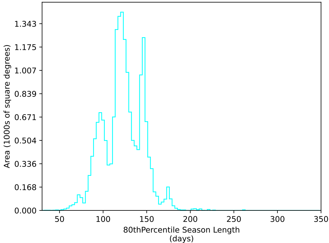
too_combined_s0.5_v3.4_10yrs WFD u band: 80thPercentile Season Length
