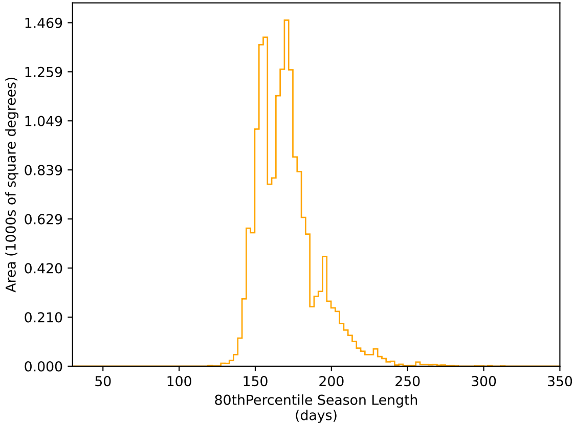
too_combined_s0.5_v3.4_10yrs WFD r band: 80thPercentile Season Length
