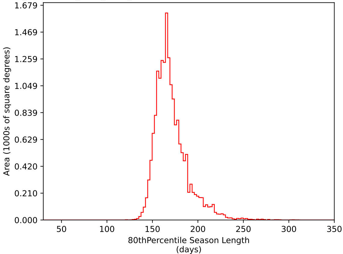
too_combined_s0.5_v3.4_10yrs WFD i band: 80thPercentile Season Length
