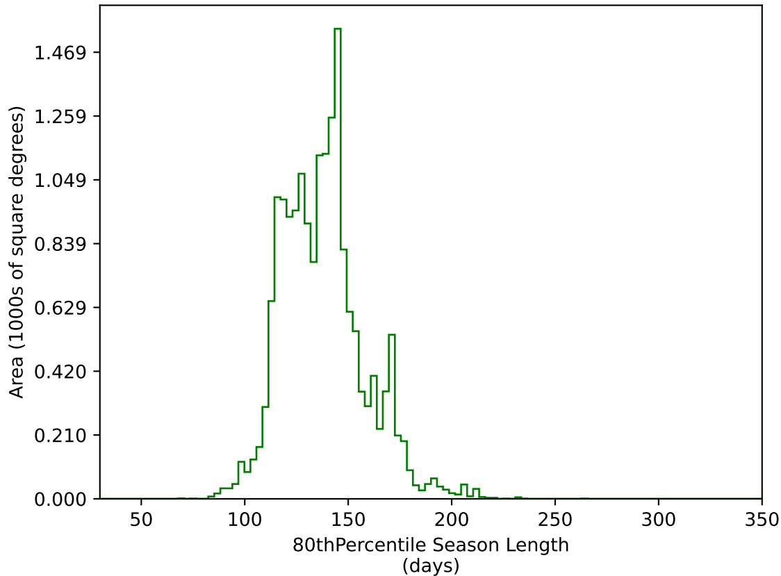
too_combined_s0.5_v3.4_10yrs WFD g band: 80thPercentile Season Length
