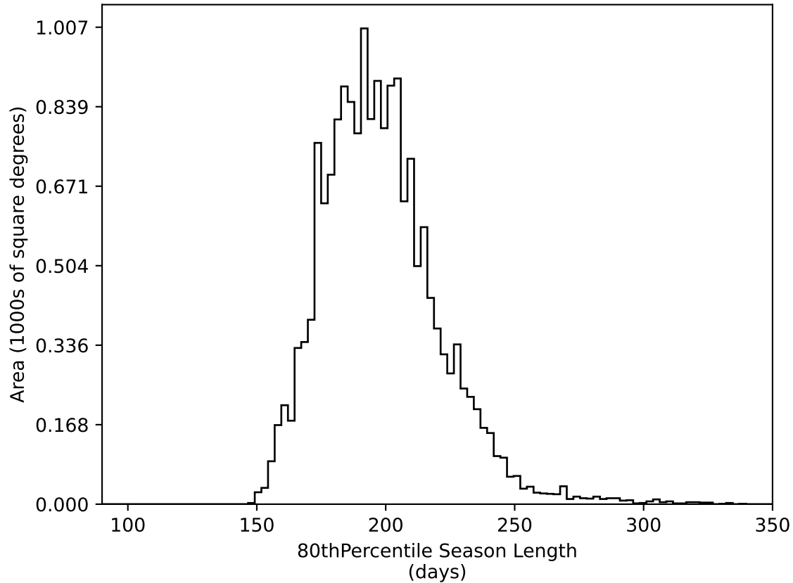
too_combined_s0.5_v3.4_10yrs WFD all bands: 80thPercentile Season Length
