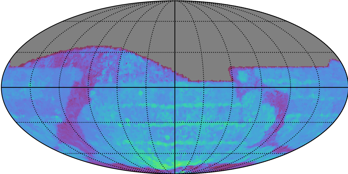
too_combined_s0.5_v3.4_10yrs All sky z band: 80thPercentile Season Length
