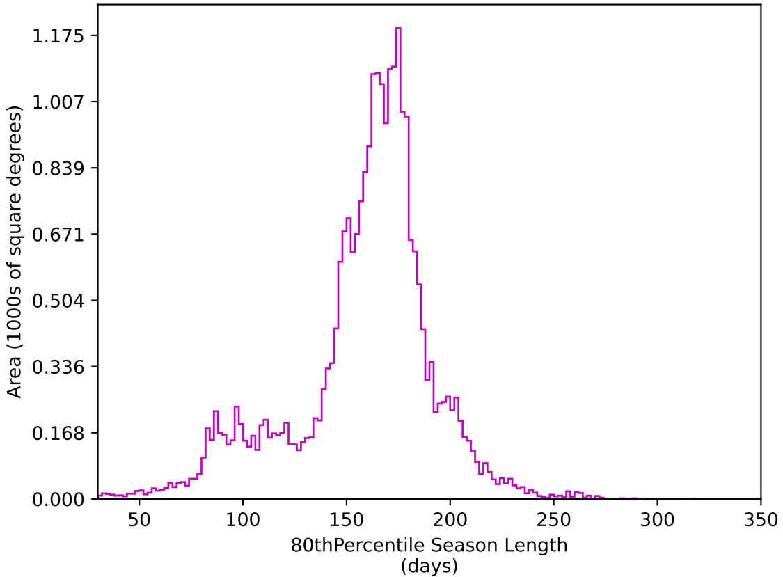
too_combined_s0.5_v3.4_10yrs All sky z band: 80thPercentile Season Length
