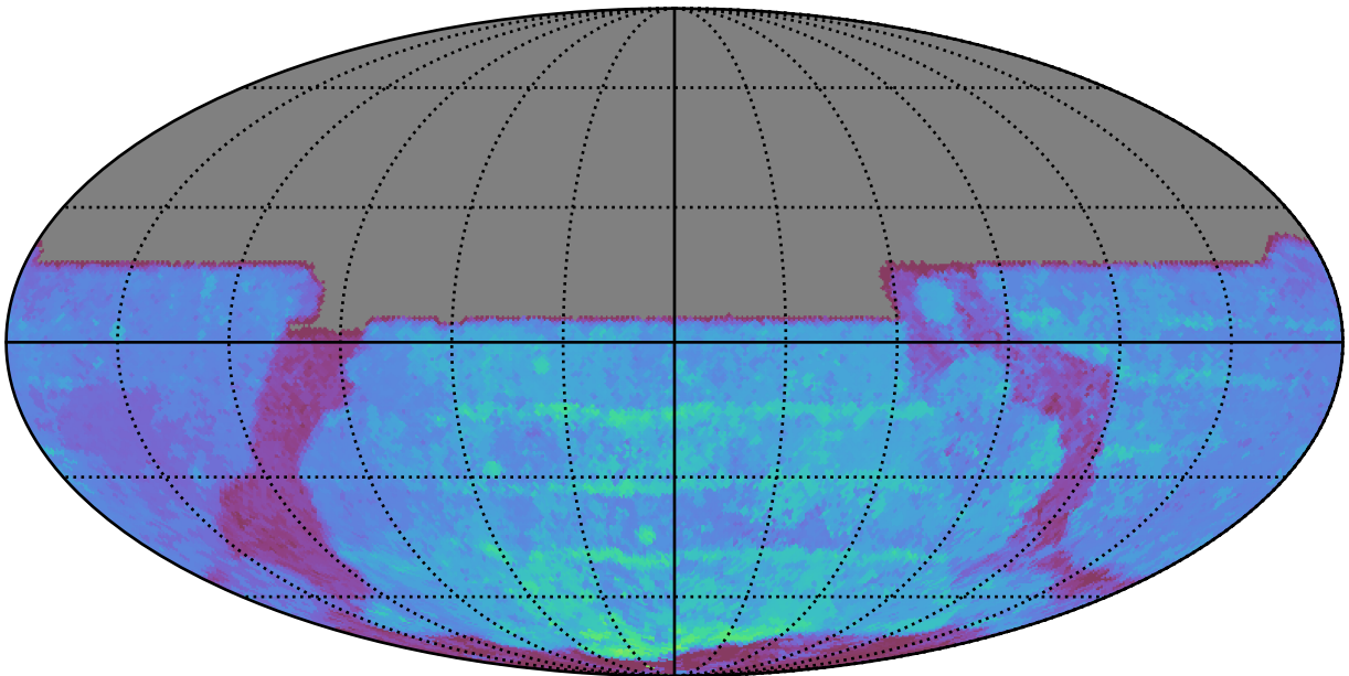
too_combined_s0.5_v3.4_10yrs All sky y band: 80thPercentile Season Length
