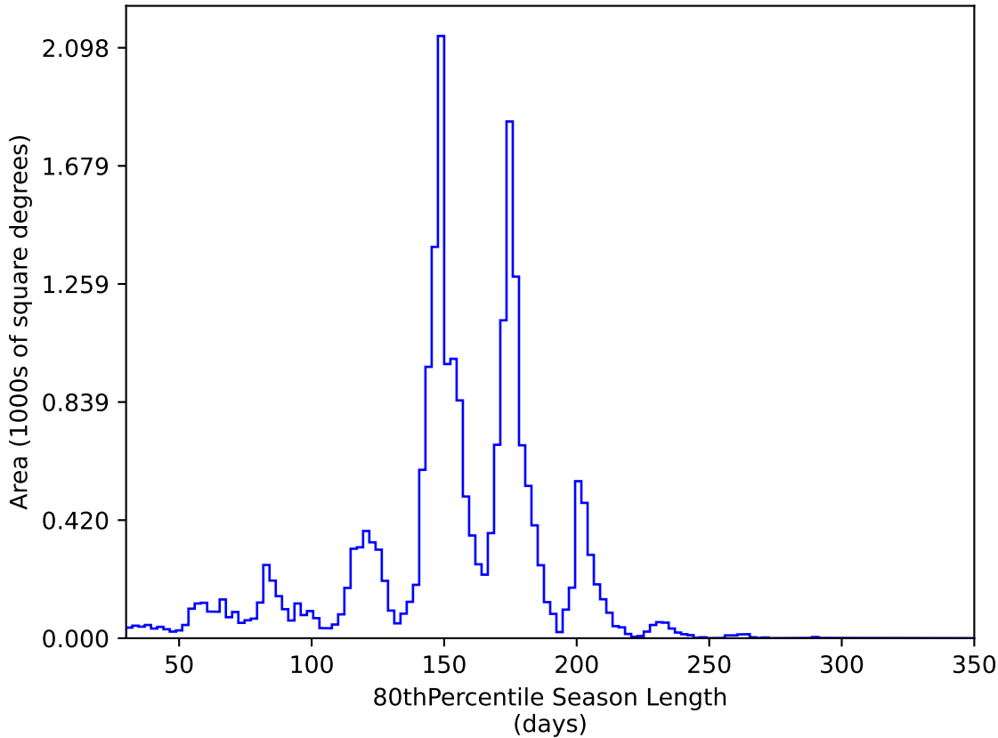
too_combined_s0.5_v3.4_10yrs All sky y band: 80thPercentile Season Length
