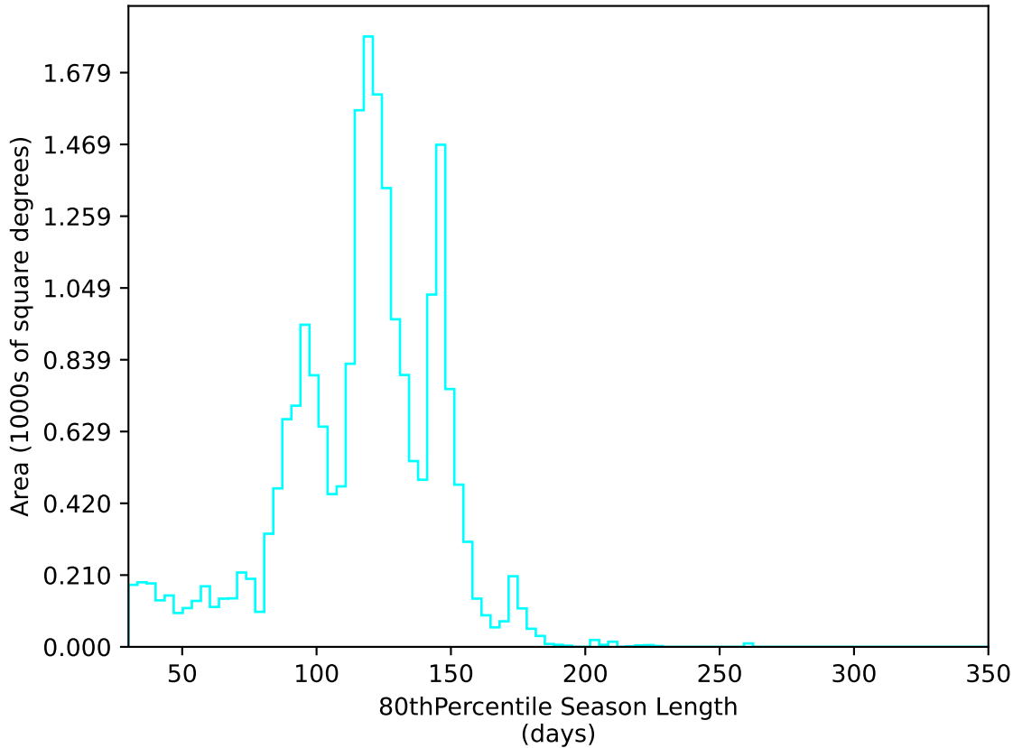
too_combined_s0.5_v3.4_10yrs All sky u band: 80thPercentile Season Length
