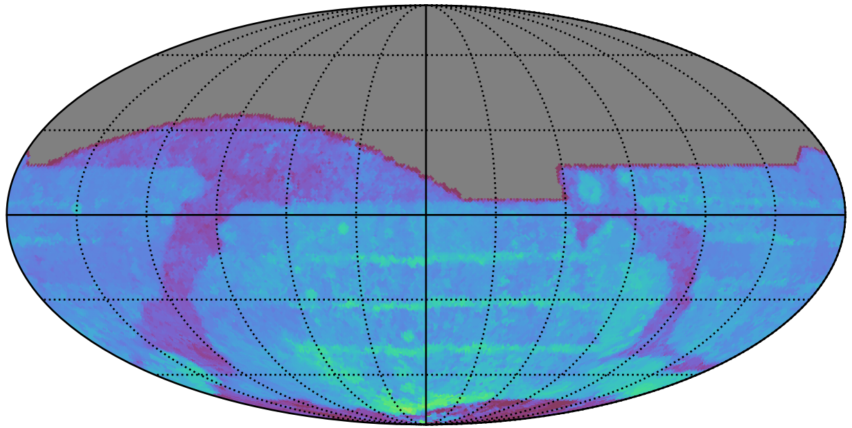
too_combined_s0.5_v3.4_10yrs All sky r band: 80thPercentile Season Length
