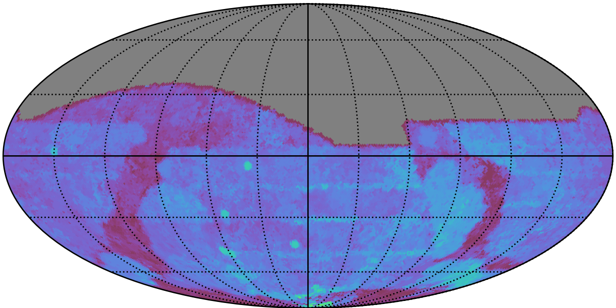
too_combined_s0.5_v3.4_10yrs All sky g band: 80thPercentile Season Length
