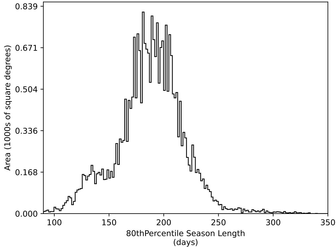
too_combined_s0.5_v3.4_10yrs All sky all bands: 80thPercentile Season Length
