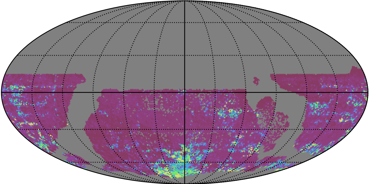
too_combined_s0.5_v3.4_10yrs WFD z band: 75th Percentile Intranight Timespan
