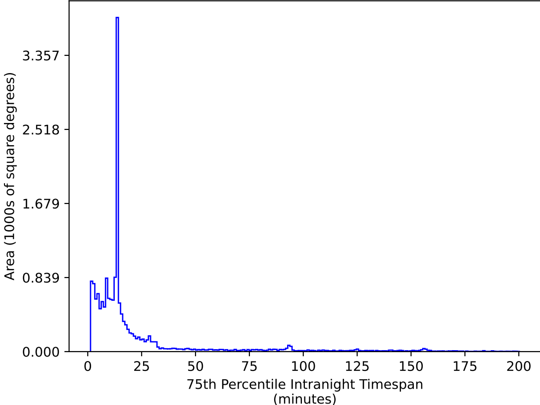
too_combined_s0.5_v3.4_10yrs WFD z band: 75th Percentile Intranight Timespan
