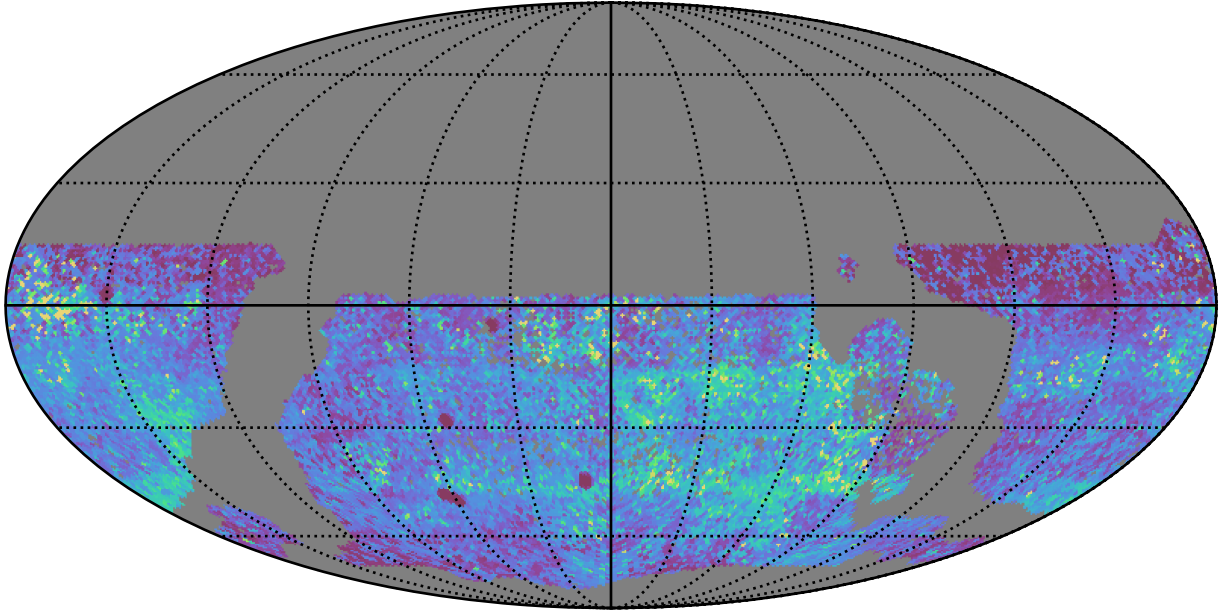
too_combined_s0.5_v3.4_10yrs WFD y band: 75th Percentile Intranight Timespan
