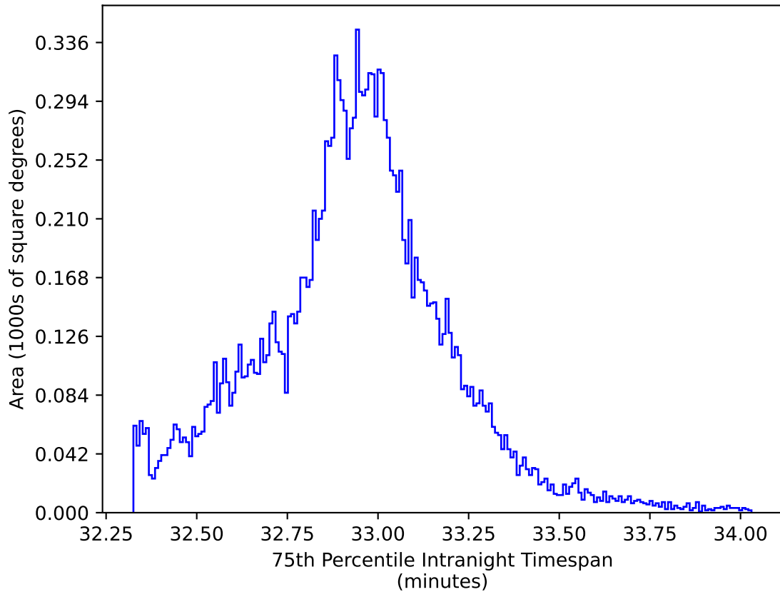
too_combined_s0.5_v3.4_10yrs WFD y band: 75th Percentile Intranight Timespan
