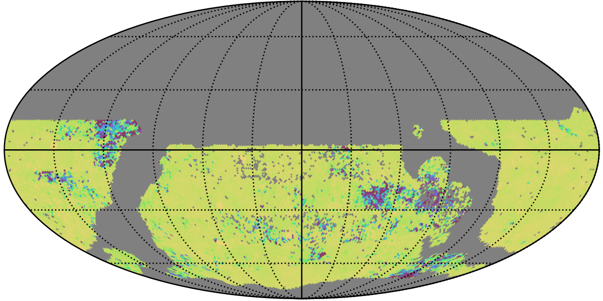
too_combined_s0.5_v3.4_10yrs WFD ug bands: 75th Percentile Intranight Timespan
