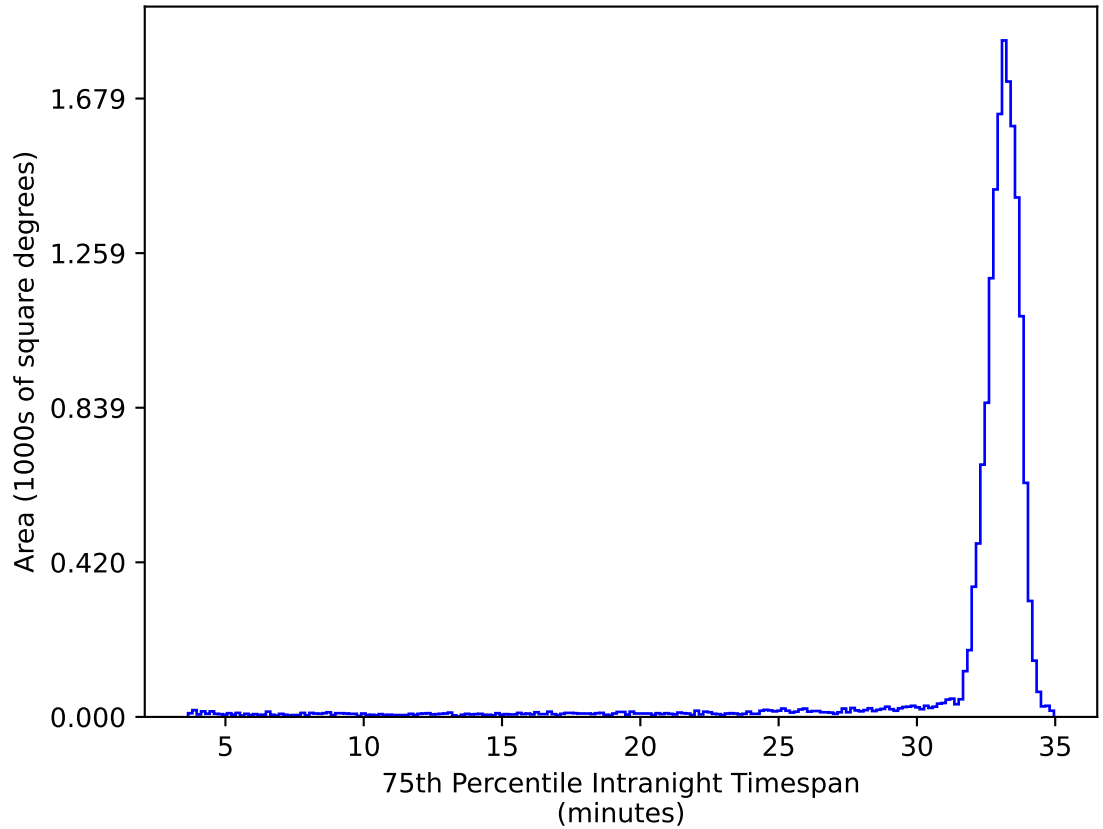
too_combined_s0.5_v3.4_10yrs WFD ug bands: 75th Percentile Intranight Timespan
