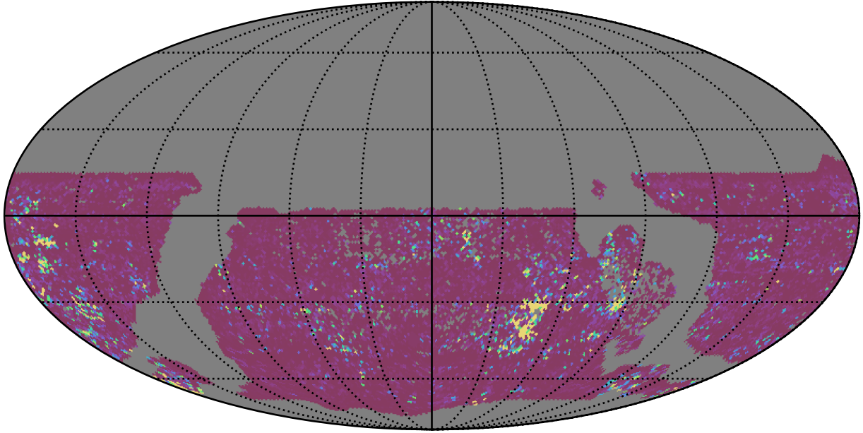
too_combined_s0.5_v3.4_10yrs WFD u band: 75th Percentile Intranight Timespan
