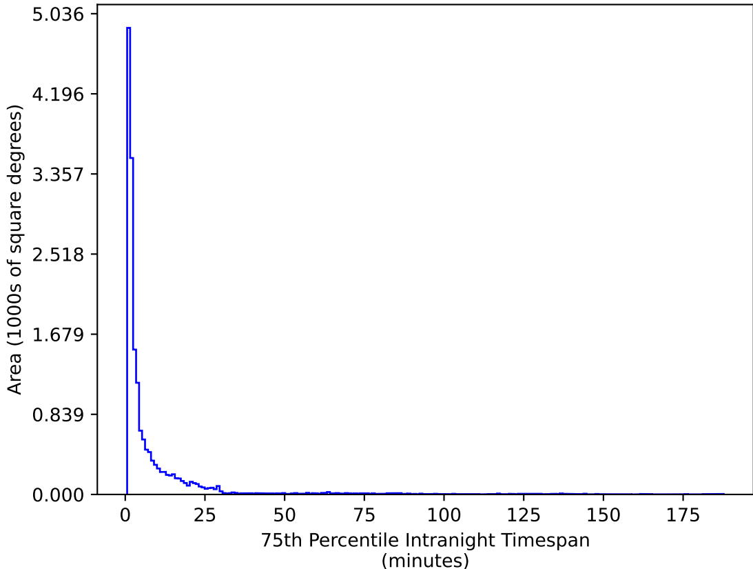
too_combined_s0.5_v3.4_10yrs WFD u band: 75th Percentile Intranight Timespan
