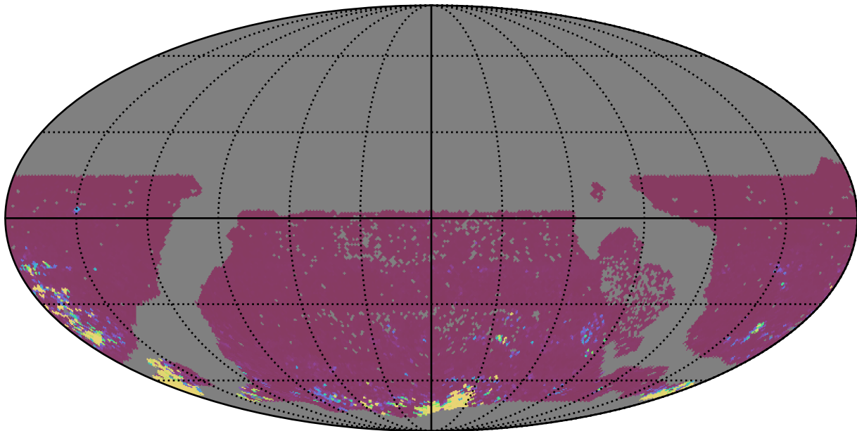
too_combined_s0.5_v3.4_10yrs WFD ri bands: 75th Percentile Intranight Timespan
