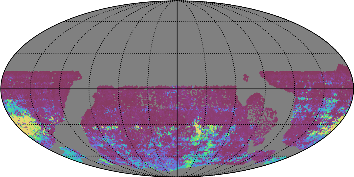
too_combined_s0.5_v3.4_10yrs WFD r band: 75th Percentile Intranight Timespan
