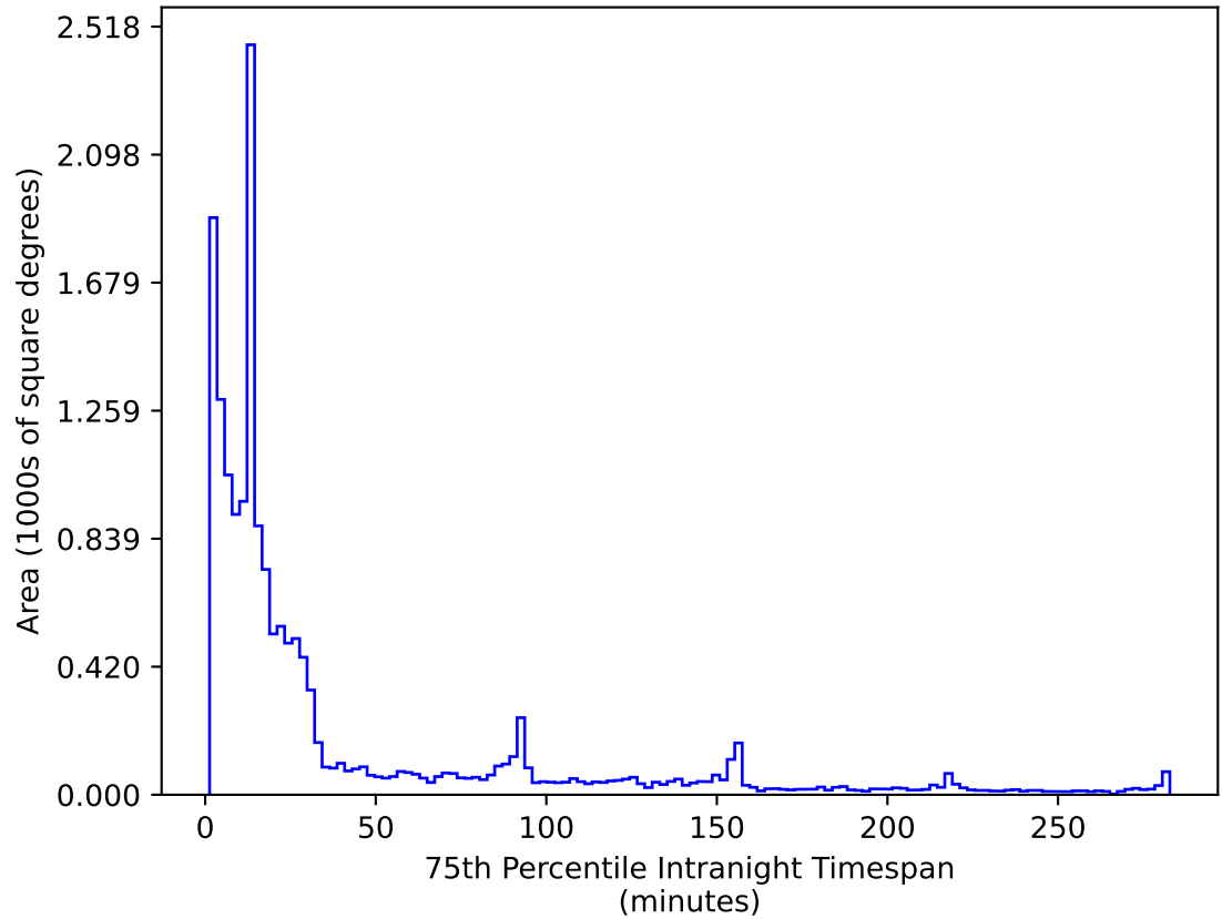
too_combined_s0.5_v3.4_10yrs WFD r band: 75th Percentile Intranight Timespan
