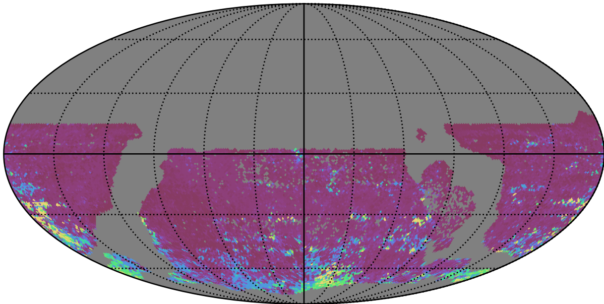
too_combined_s0.5_v3.4_10yrs WFD i band: 75th Percentile Intranight Timespan
