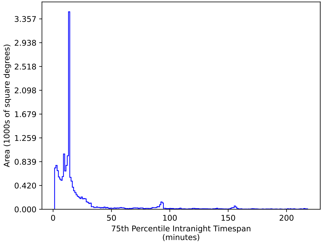
too_combined_s0.5_v3.4_10yrs WFD i band: 75th Percentile Intranight Timespan
