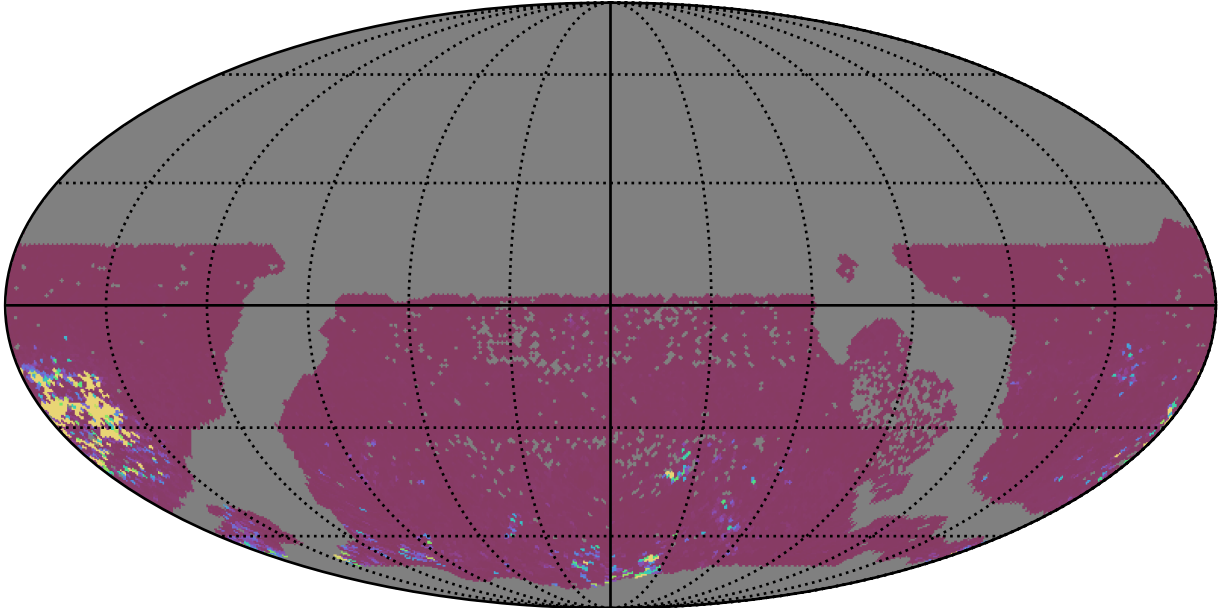
too_combined_s0.5_v3.4_10yrs WFD gr bands: 75th Percentile Intranight Timespan
