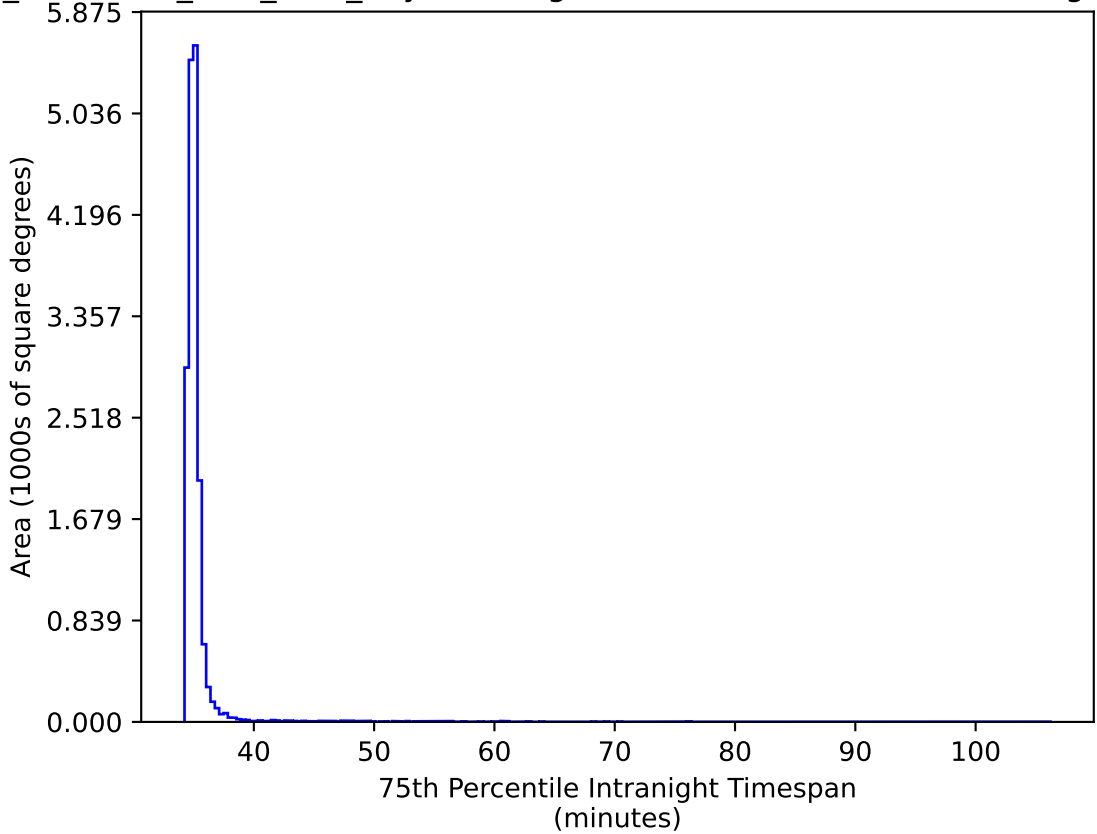
too_combined_s0.5_v3.4_10yrs WFD gr bands: 75th Percentile Intranight Timespan
