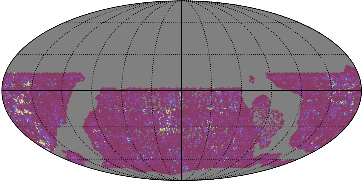
too_combined_s0.5_v3.4_10yrs WFD g band: 75th Percentile Intranight Timespan
