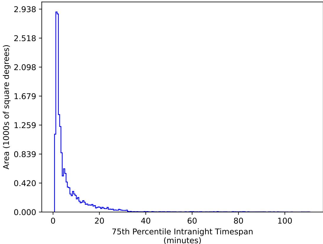
too_combined_s0.5_v3.4_10yrs WFD g band: 75th Percentile Intranight Timespan
