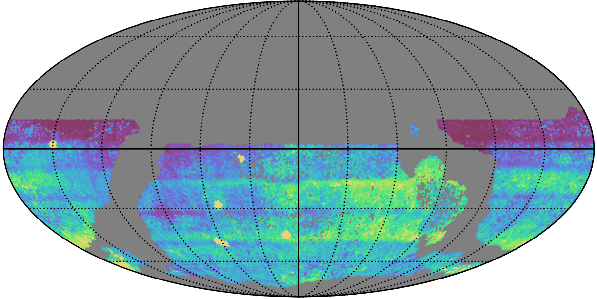
too_combined_s0.5_v3.4_10yrs WFD all bands: 75th Percentile Intranight Timespan
