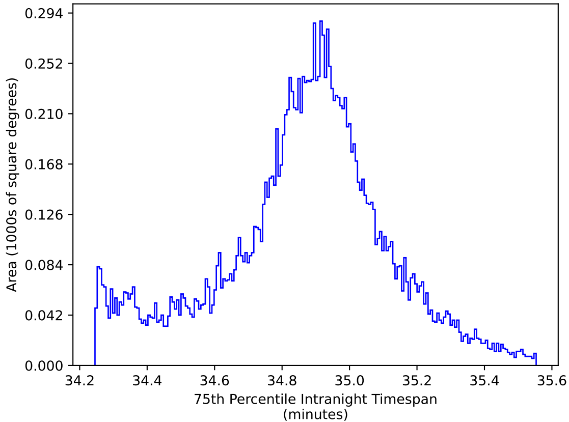
too_combined_s0.5_v3.4_10yrs WFD all bands: 75th Percentile Intranight Timespan
