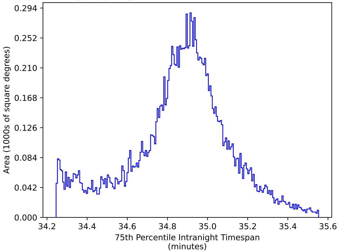
too_combined_s0.5_v3.4_10yrs WFD: 75th Percentile Intranight Timespan
