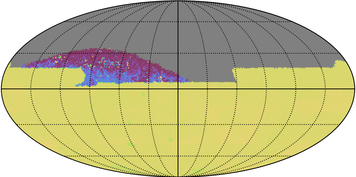
too_combined_s0.5_v3.4_10yrs All sky zy bands: 75th Percentile Intranight Timespan
