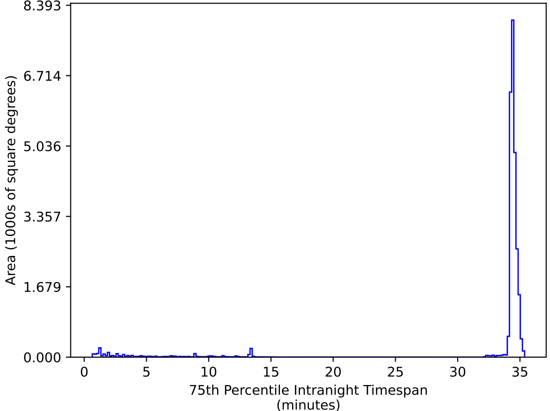
too_combined_s0.5_v3.4_10yrs All sky zy bands: 75th Percentile Intranight Timespan
