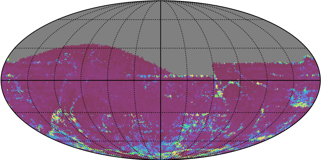
too_combined_s0.5_v3.4_10yrs All sky z band: 75th Percentile Intranight Timespan
