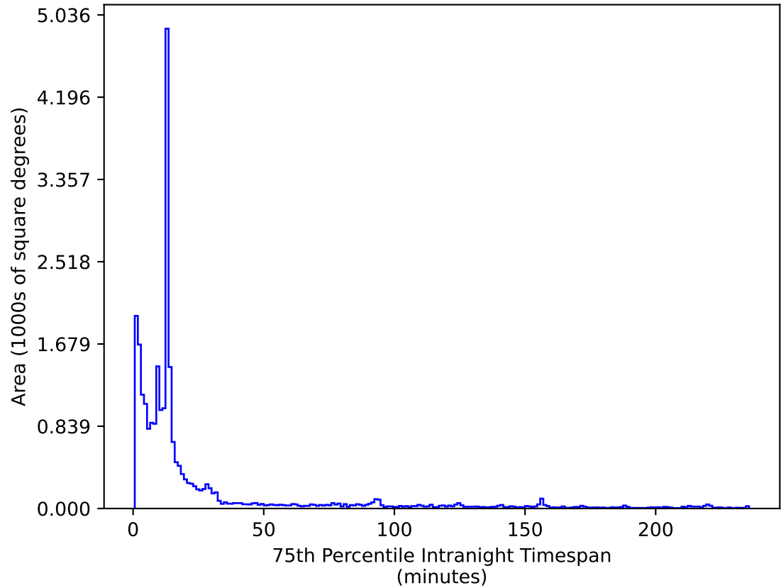
too_combined_s0.5_v3.4_10yrs All sky z band: 75th Percentile Intranight Timespan
