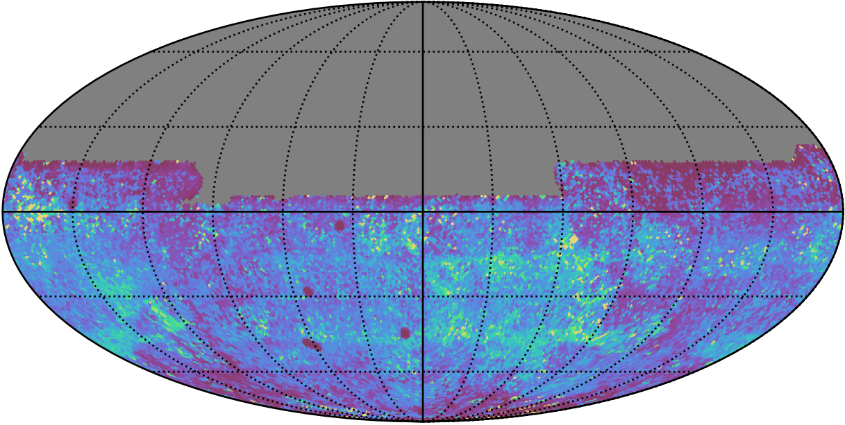
too_combined_s0.5_v3.4_10yrs All sky y band: 75th Percentile Intranight Timespan
