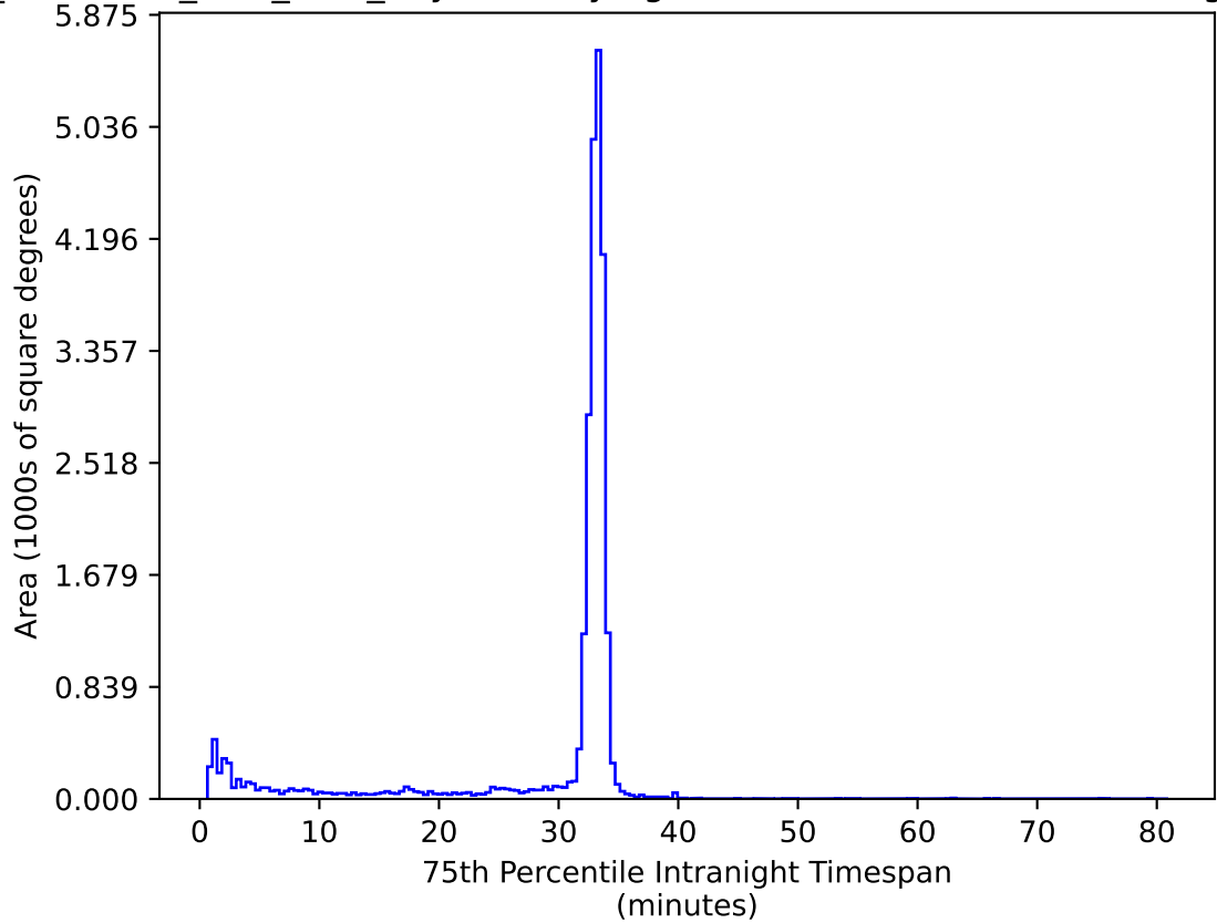
too_combined_s0.5_v3.4_10yrs All sky ug bands: 75th Percentile Intranight Timespan
