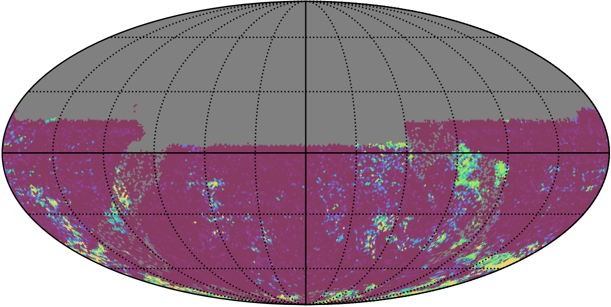
too_combined_s0.5_v3.4_10yrs All sky u band: 75th Percentile Intranight Timespan
