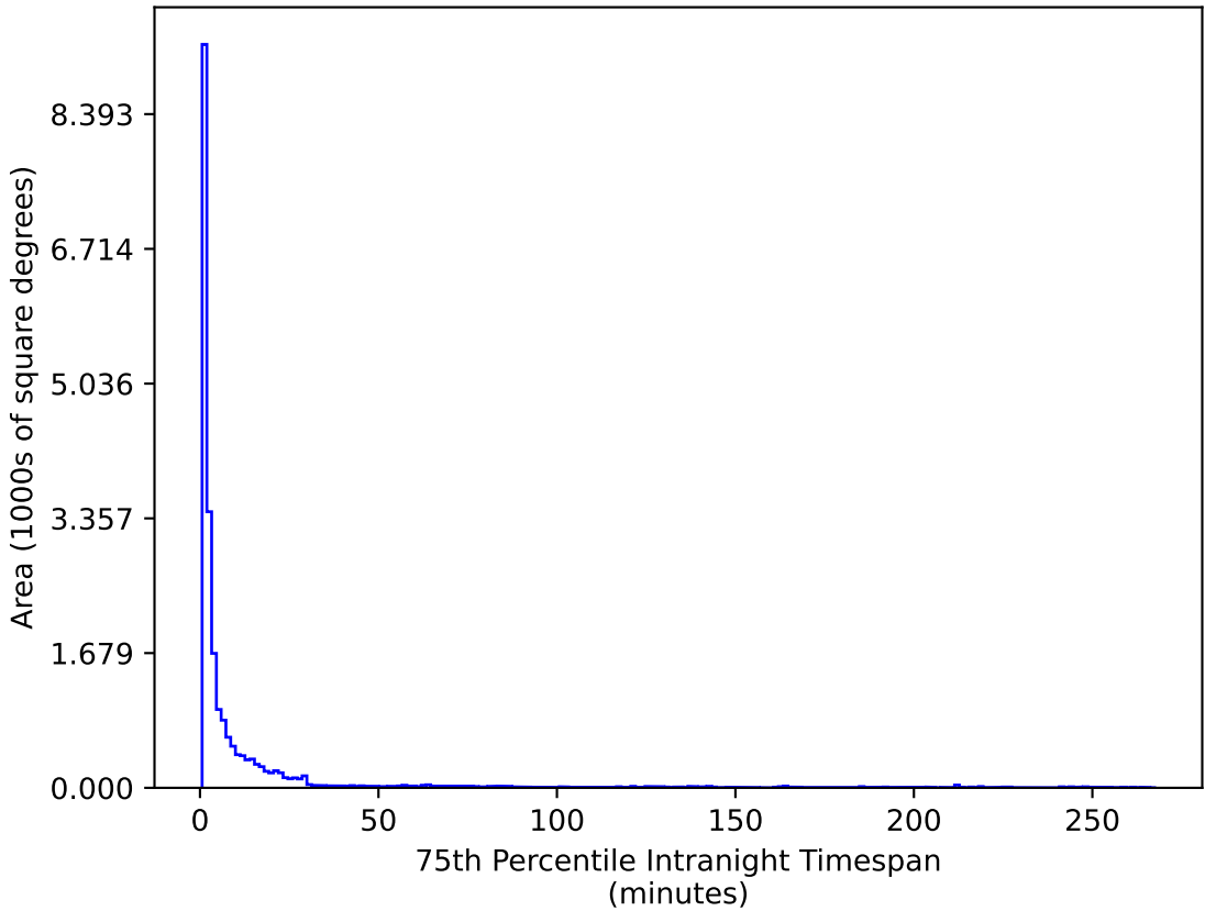
too_combined_s0.5_v3.4_10yrs All sky u band: 75th Percentile Intranight Timespan
