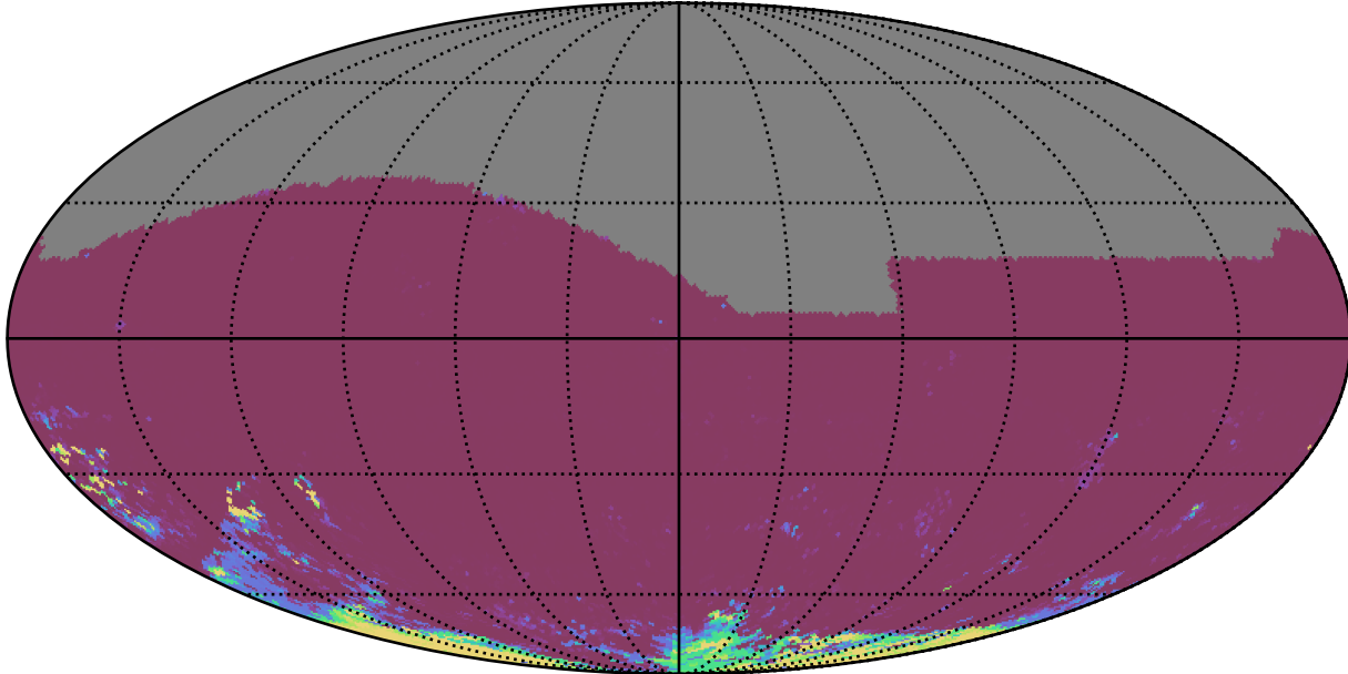
too_combined_s0.5_v3.4_10yrs All sky ri bands: 75th Percentile Intranight Timespan
