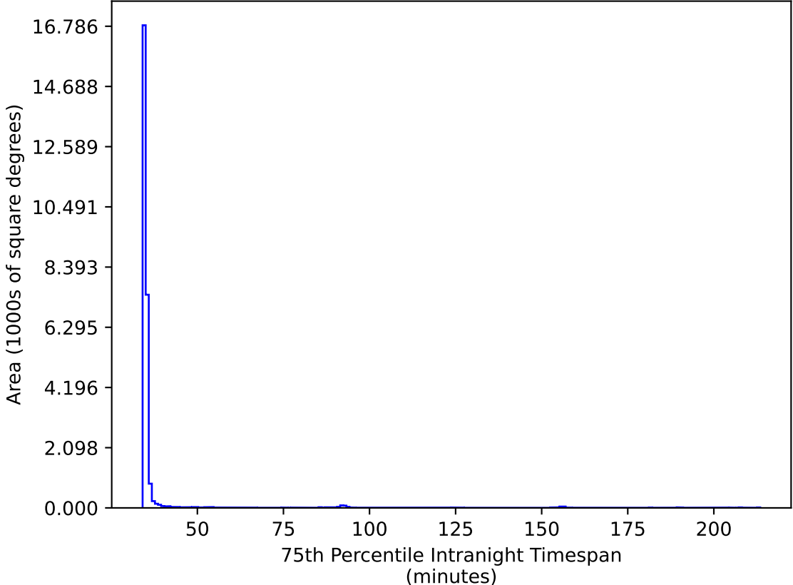
too_combined_s0.5_v3.4_10yrs All sky ri bands: 75th Percentile Intranight Timespan
