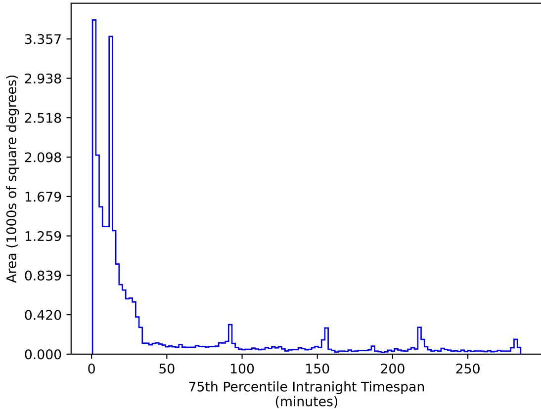
too_combined_s0.5_v3.4_10yrs All sky r band: 75th Percentile Intranight Timespan
