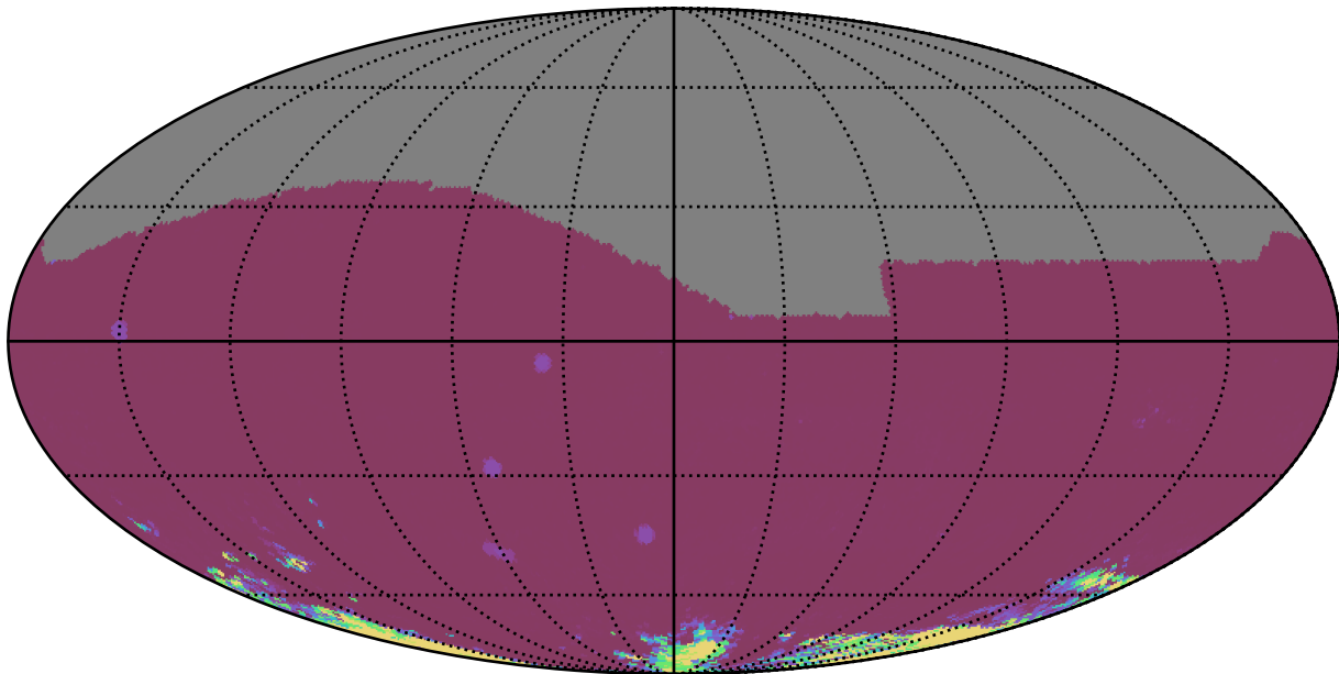
too_combined_s0.5_v3.4_10yrs All sky iz bands: 75th Percentile Intranight Timespan
